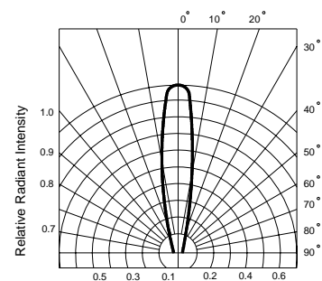
FIG.6 Radiant Diagram
