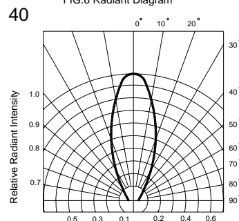
FIG.6 Radiant Diagram
