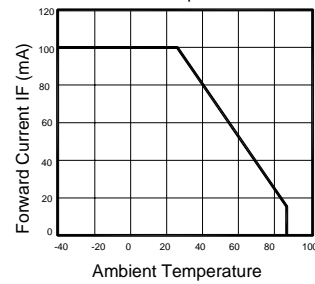
Fig.2 Forward Current Vs Ambient Temperature
